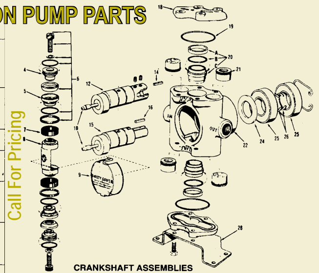
CRANKSHAFT ASSEMBLIES
