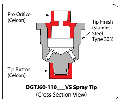
DGTJ60-110 VS Spray Tip (Cross Section View)
